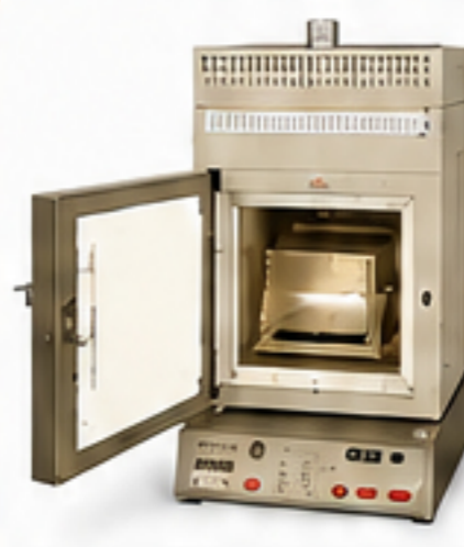
Asphalt ignition oven
